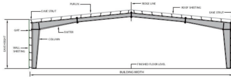
TYPICAL ELEVATION
