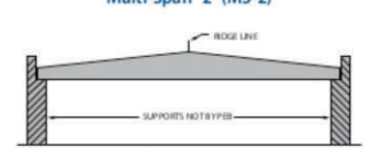
MAX. PRACTICAL WIDTH = 50 m Roof System (RS)
