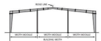
MAX. PRACTICAL WIDTH = 200 m Multi-Span "2" (MS-2)
